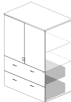
ST-L-36##-2L-R (Lock Right)
